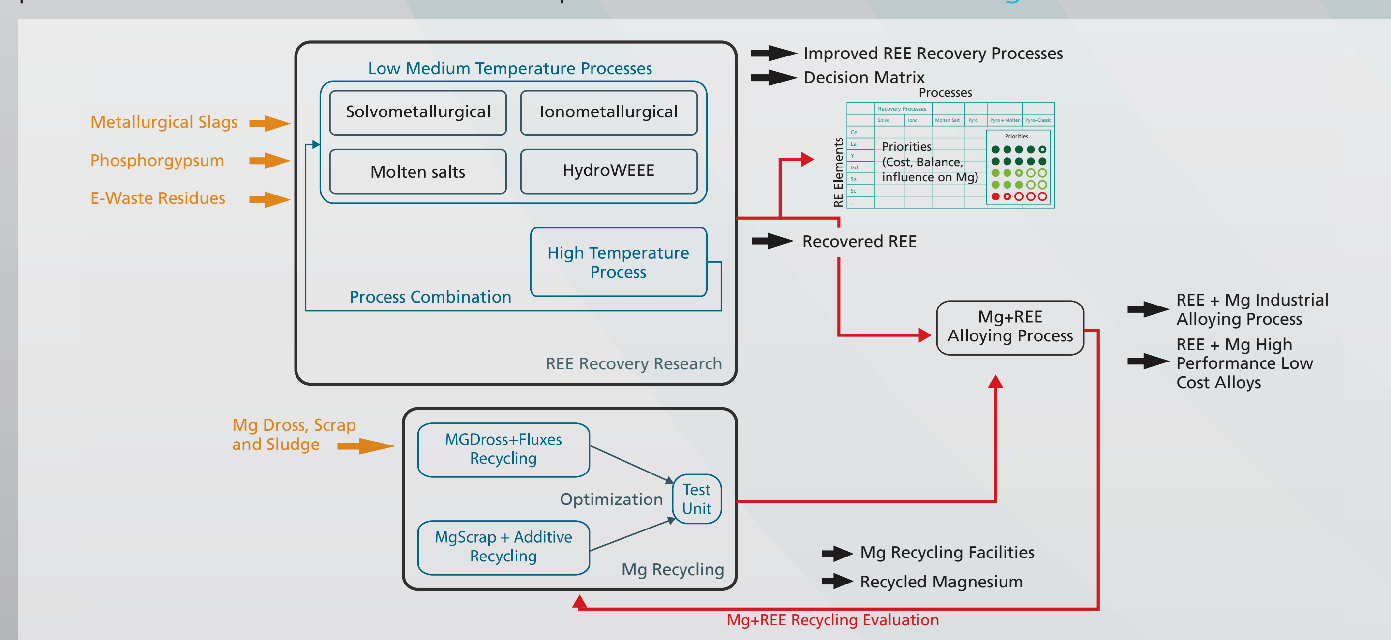
Fig.1: Process evaluation and industrialization flow chart
